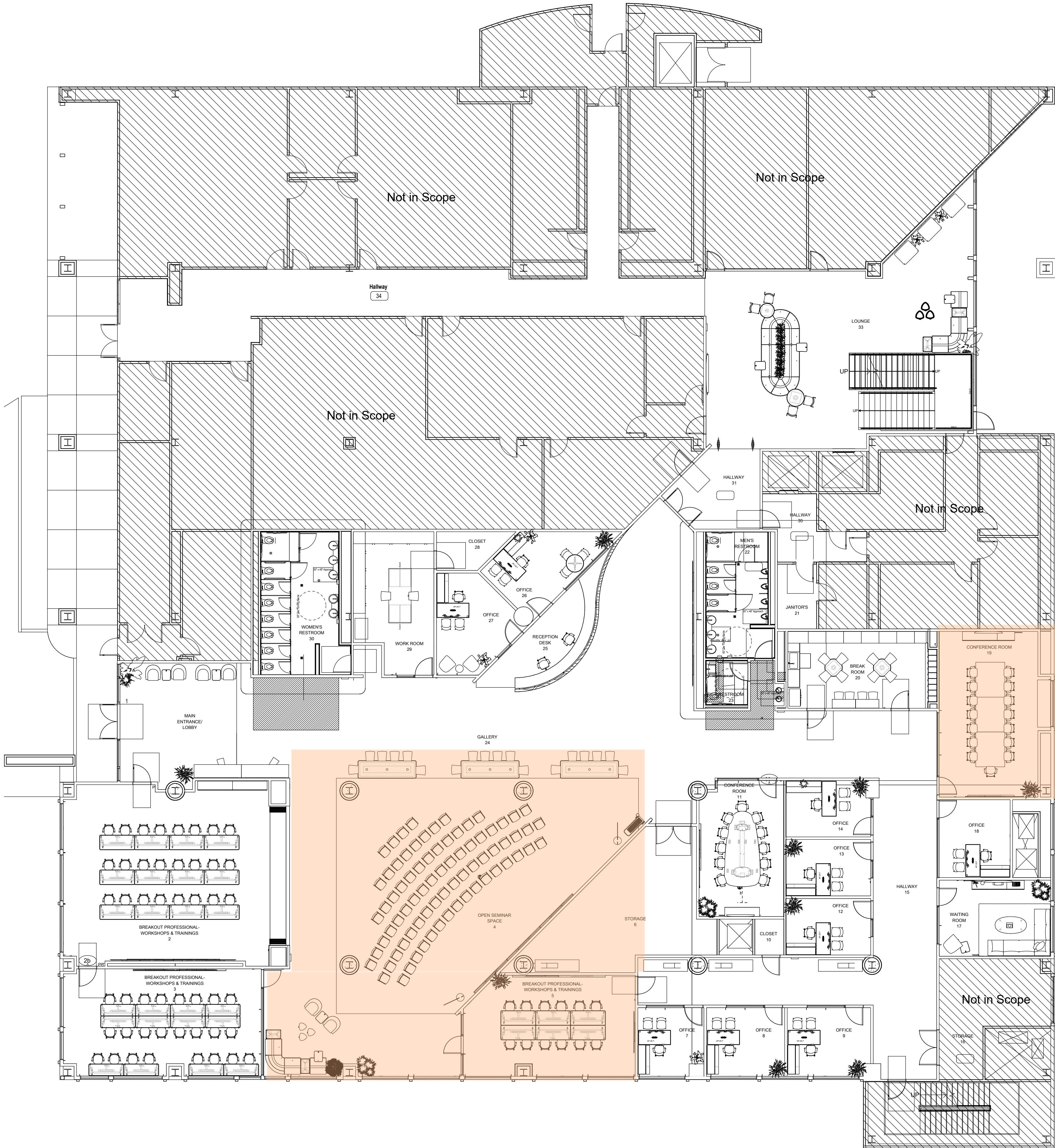
OVERALL PLAN VIEW
